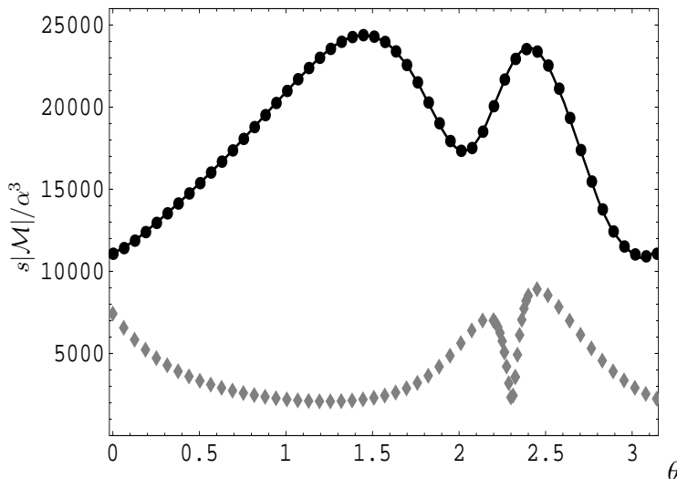
Figure 1: Comparison with figure 5 of ref. [19]. Helicity configurations [+ + - - - -] and [+ - - + + -] for the momenta of eq. (4.1), represented by black dots and gray diamonds respectively, and comparison with the analytic result of ref. [18] (continuous line).
