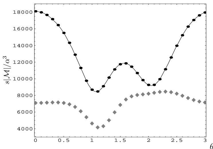
Figure 2: Helicity configurations [+ + - - - -] and [+ + - - + -] for the momenta of eq. (4.2), represented by black dots and gray diamonds respectively, and comparison with the analytic result of ref. [18] (continuous line).
